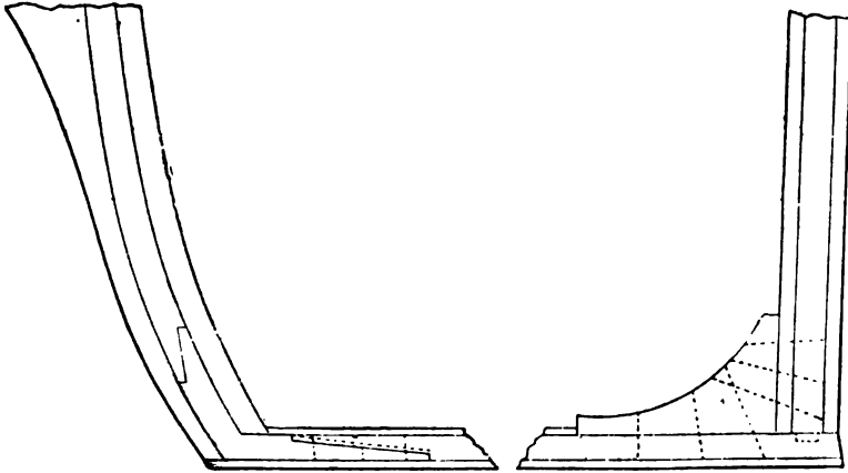
Fig. 334.—Longitudinal section of a ship. (After Boppe.)
